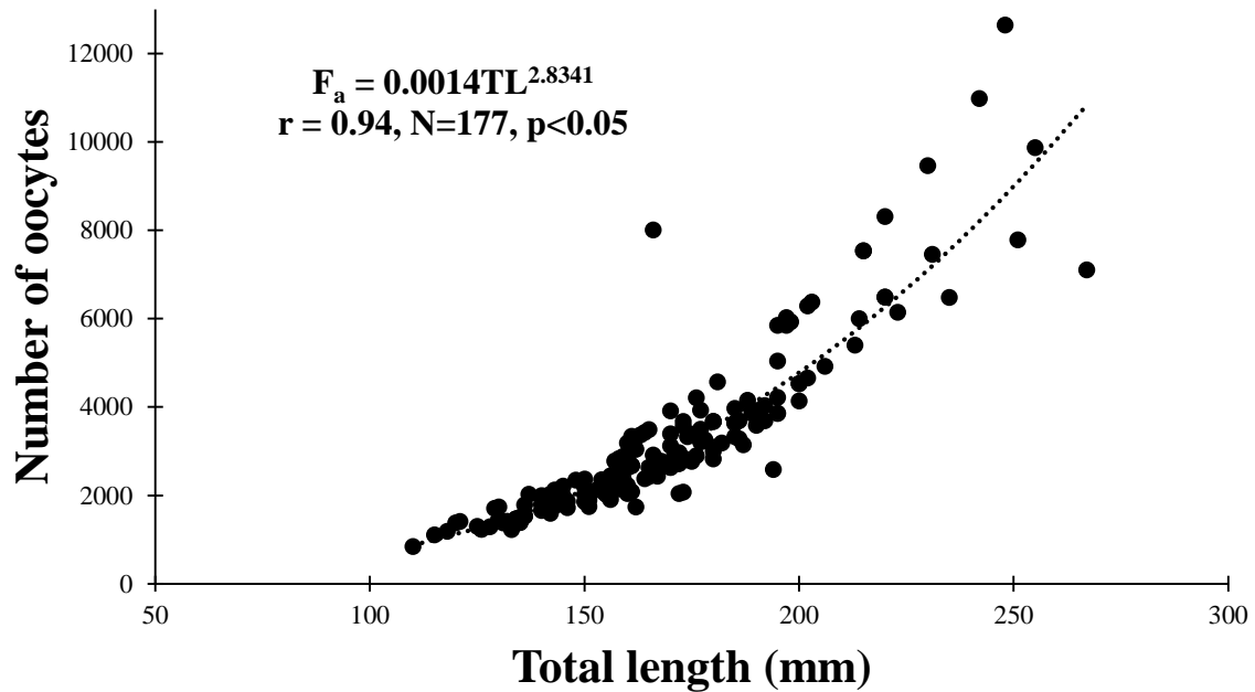
Fig. 8: Power function between fecundity ( F_a ) and total length (TL) of Marcusenius senegalensis collected in Niger River (Northern Benin) from February 2015 to July 2016.
