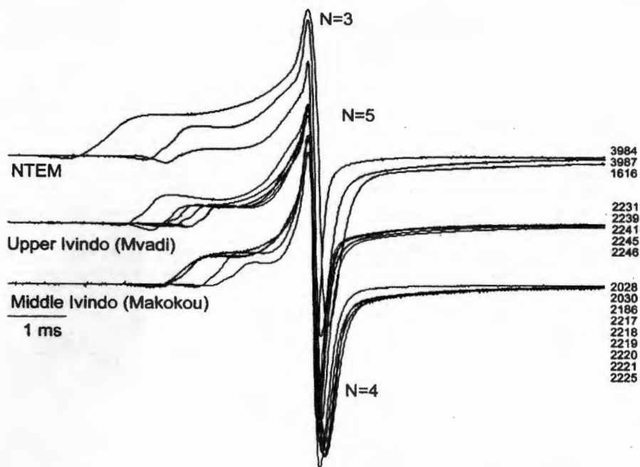
Fig. 5. - Electric organ discharges recorded from M. ntemensis / M. conicephalus from the Ntem and Ivindo River basins. Code numbers refer to individual field identification numbers.
